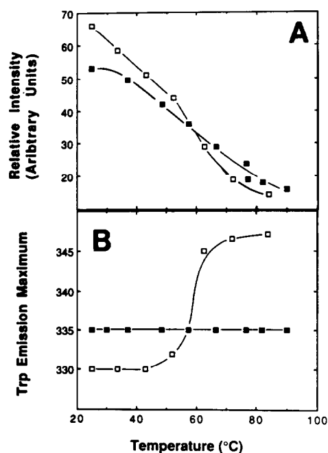
Fig.2. Change in tryptophan (A) fluorescence intensity and (B) emission maximum of \alpha_L (solid squares) and \beta B2 (open squares) as a function of temperature. Protein concentrations of both were 0.1 mg/ml in 0.1 M phosphate buffer, pH 7.4.
